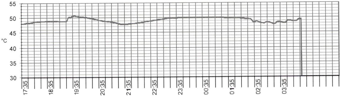
Temperature / Time graph - Temperature during exposure time : min 47,7 / MAX 49,9 °C
