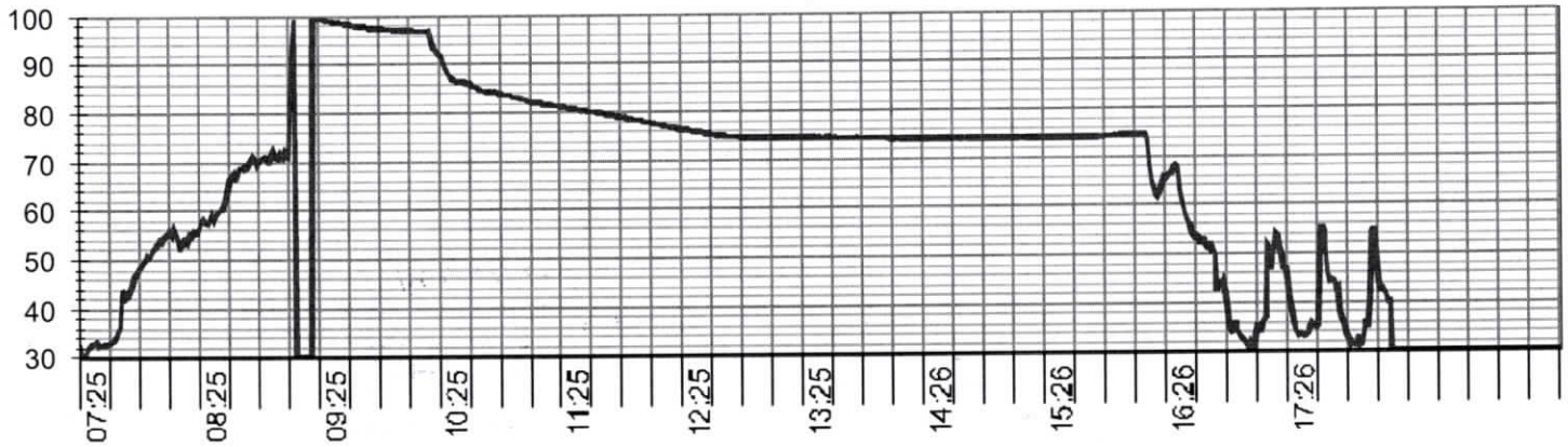
Relative humidity / Time graph - RH at the end of conditioning : 71 %, RH during exposure time : min 74 %
