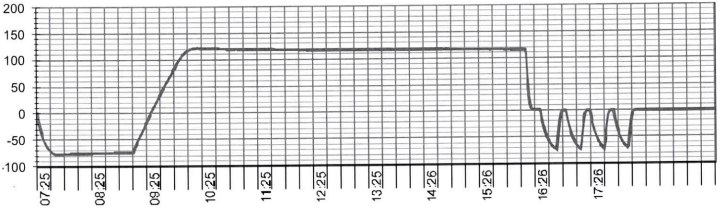
Pressure / Time graph - Pressure during exposure time : min 116 / MAX 122 kPa
