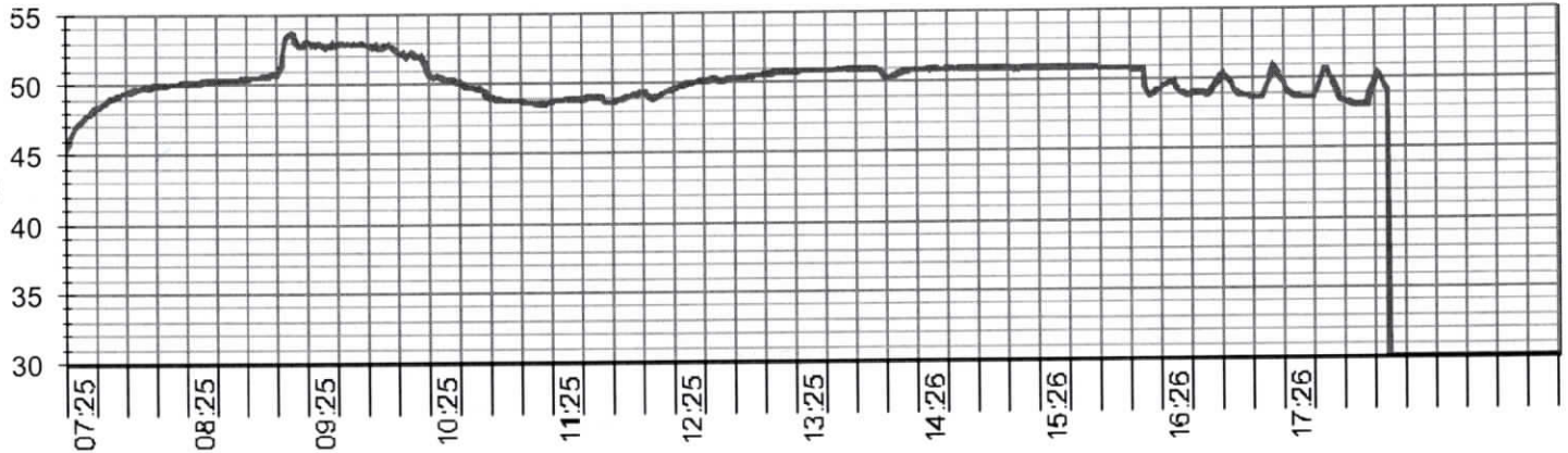
Temperature / Time graph - Temperature during exposure time : min 48,5 / MAX 52,0 °C
