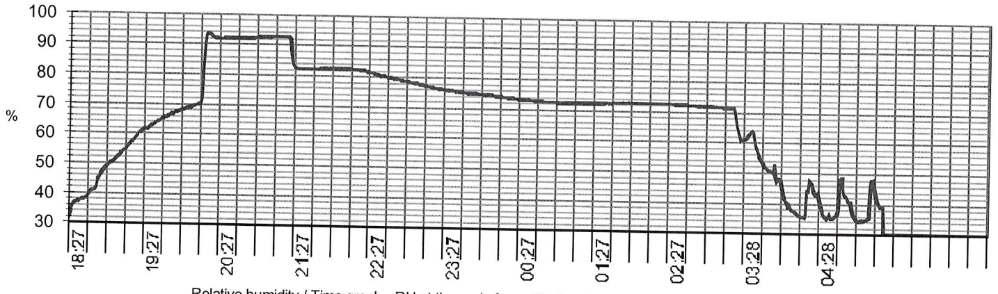
Relative humidity / Time graph - RH at the end of conditioning : 70 %, RH during exposure time : min 71 %
