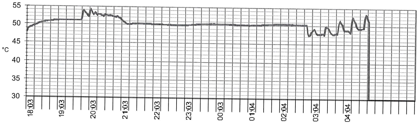
Temperature / Time graph - Temperature during exposure time : min 49,9 / MAX 51,9 °C
