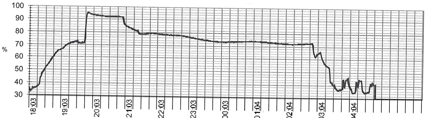
Relative humidity / Time graph - RH at the end of conditioning : 72 %, RH during exposure time : min 72 %
