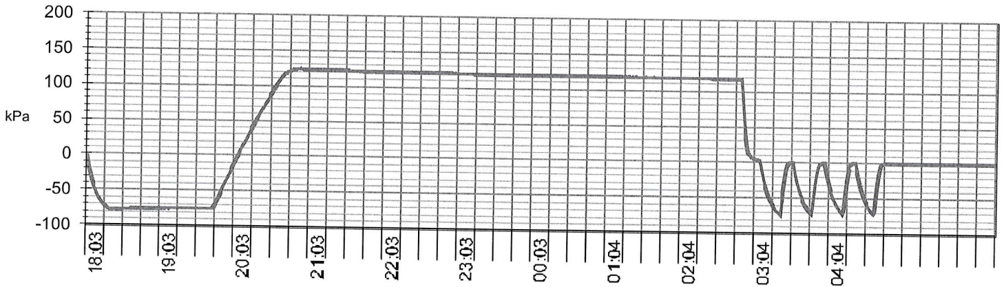
Pressure / Time graph - Pressure during exposure time : min 118 / MAX 124 kPa
