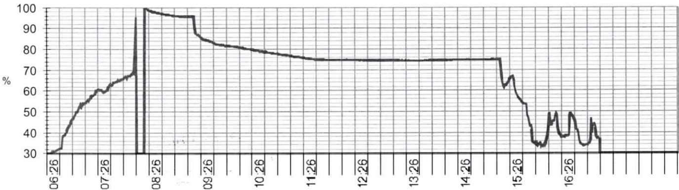
Relative humidity / Time graph - RH at the end of conditioning : 69 %, RH during exposure time : min 74 %
