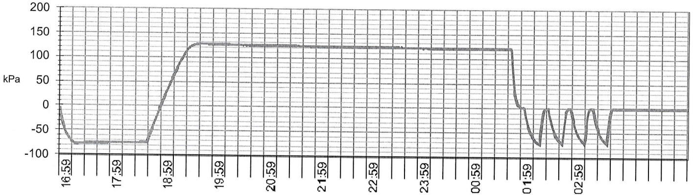
Pressure / Time graph - Pressure during exposure time : min 121 / MAX 126 kPa
