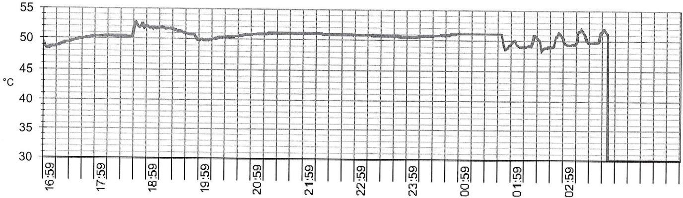
Temperature / Time graph - Temperature during exposure time : min 49,7 / MAX 51,1 °C
