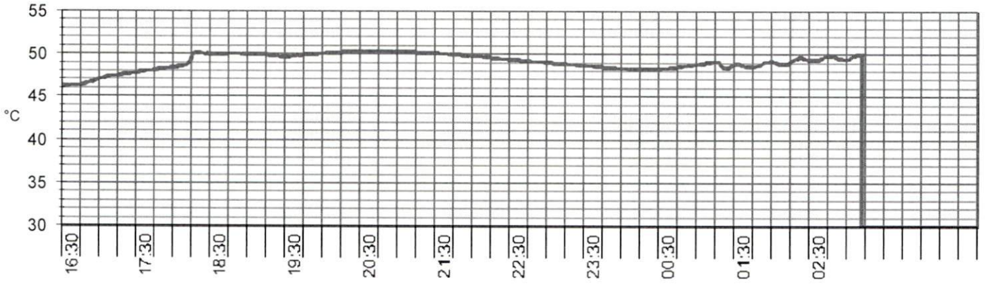
Temperature / Time graph - Temperature during exposure time : min 48,2 / MAX 50,3 °C
