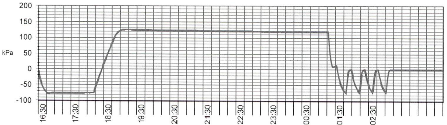
Pressure / Time graph - Pressure during exposure time : min 119 / MAX 125 kPa
