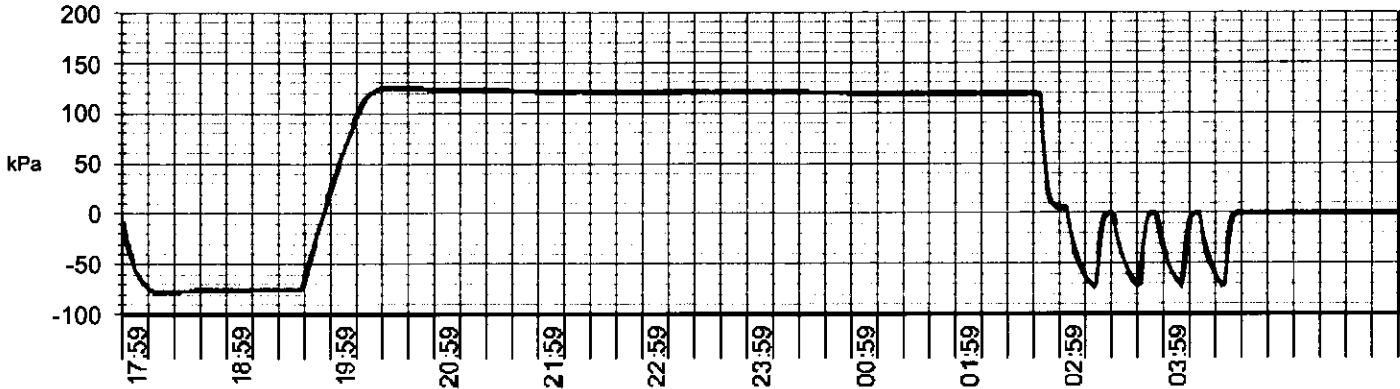
Pressure / Time graph - Pressure during exposure time : min 118 / MAX 124 kPa
