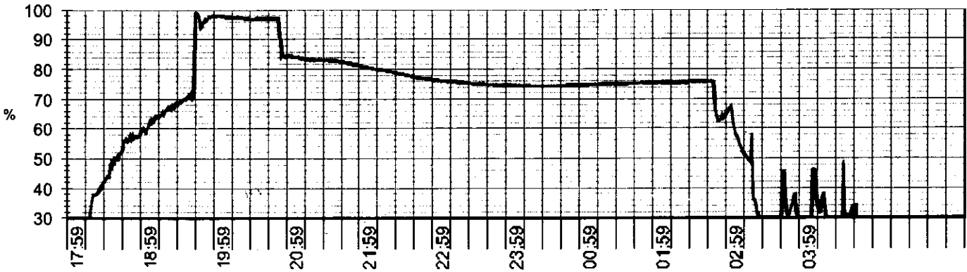
Relative humidity / Time graph - RH at the end of conditioning : 72 %, RH during exposure time : min 74 %
