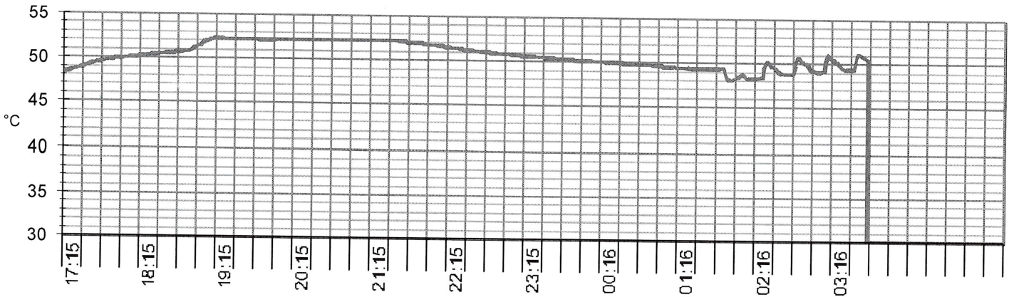
Temperature / Time graph - Temperature during exposure time : min 49,3 / MAX 52,2 °C
