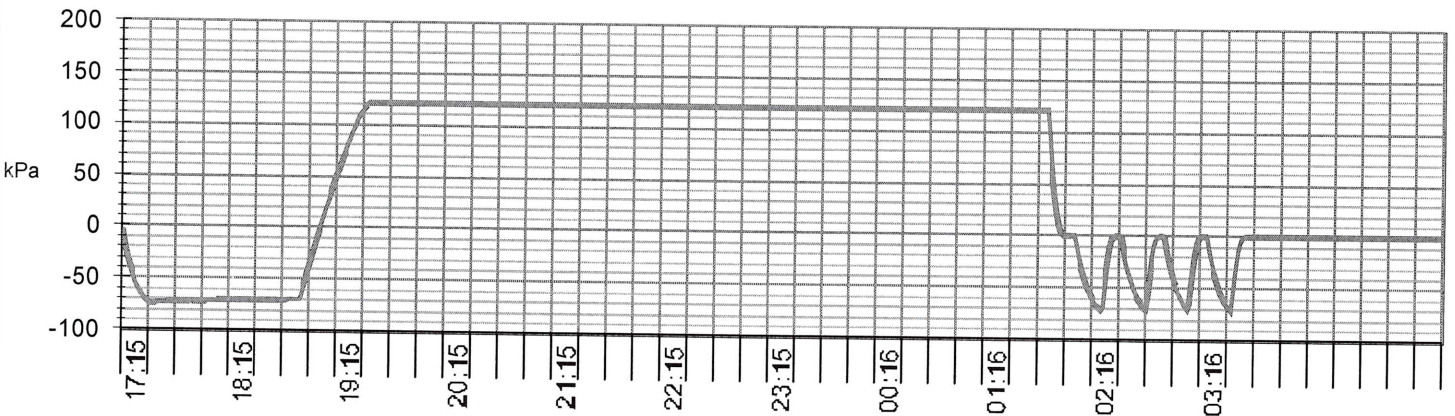
Pressure / Time graph - Pressure during exposure time : min 120 / MAX 120 kPa
