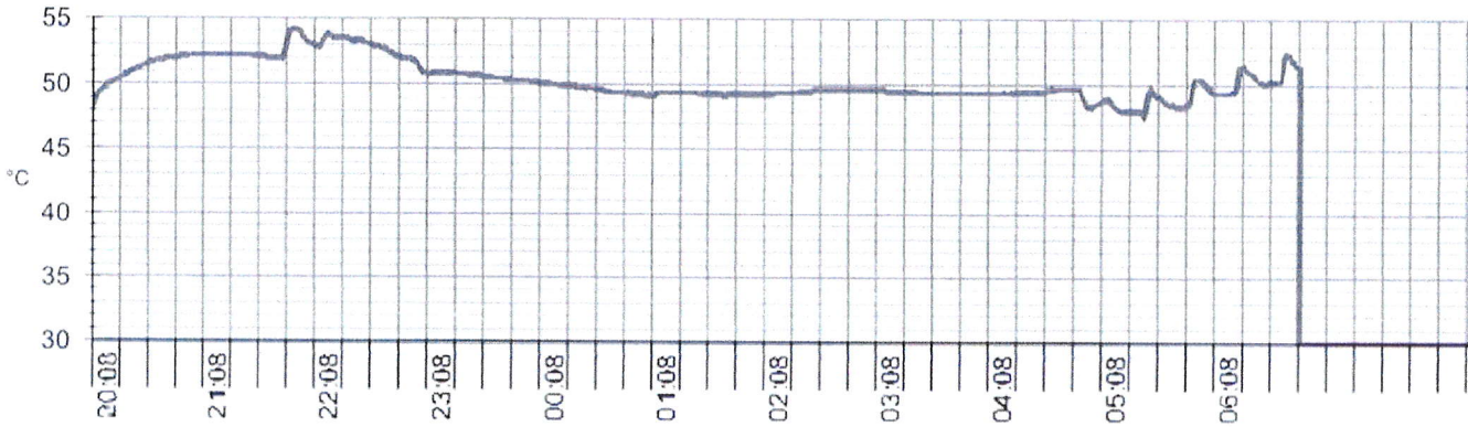
Temperature / Time graph - Temperature during exposure time : min 49,2 / MAX 51,8 °C
